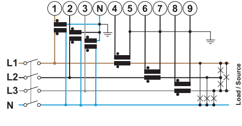
3 Phases, 4 Wires - VT/CT
